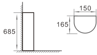
ATLANTIS BASIN PEDESTAL - FULL
