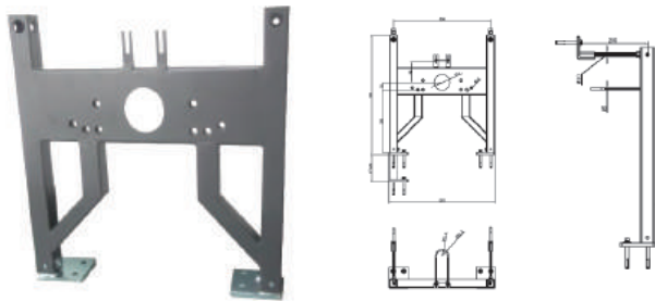
NOVATEC UNIVERSAL CHAIR BRACKET FOR WALL HUNG WC
