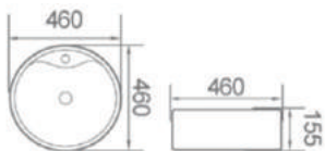
ATLANTIS COUNTER TOP BASIN
