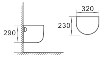
ATLANTIS BASIN PEDESTAL - HALF
