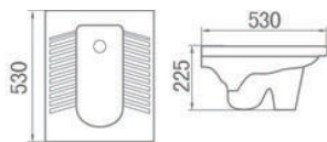
ATLANTIS RECTANGULAR SQUATTING PAN
