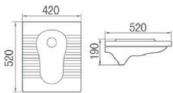
ATLANTIS RECTANGULAR SQUATTING PAN
