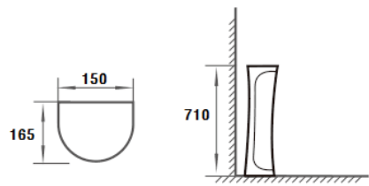
ATLANTIS BASIN PEDESTAL - FULL
